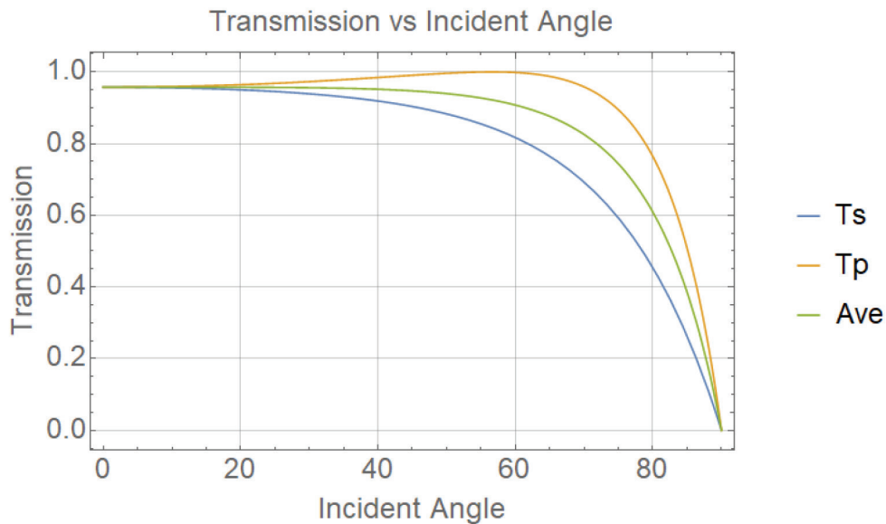
Figure 4. Fresnel transmission coefficient for S and P polarizations and their average.
